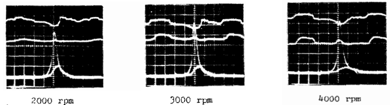
Fig. 9 - Movement of strong L-ring (as a top ring) under full load
