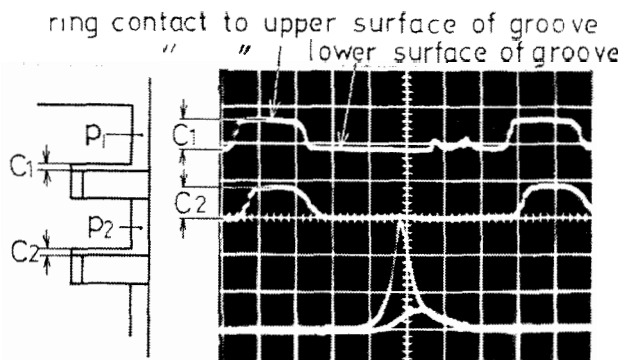
Fig. 7 - Typical record with rectangular rings
